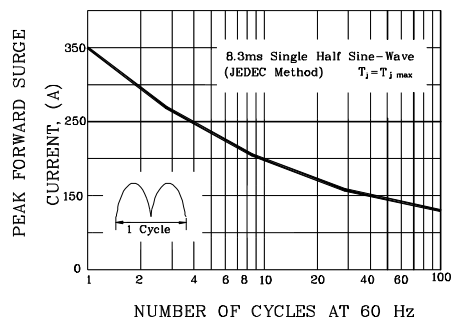
FIG.2-MAXIMUM NON-REPETITIVE PEAK FORWARD SURGE CURRENT PER ELEMENT
